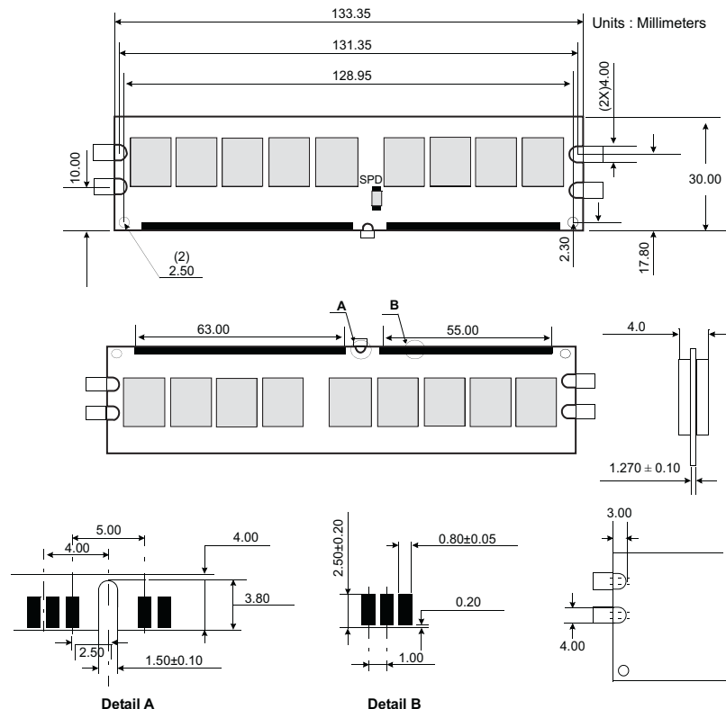
Figure 1: KVR533D2E4K2/2G 240-Pin DIMM Kit
